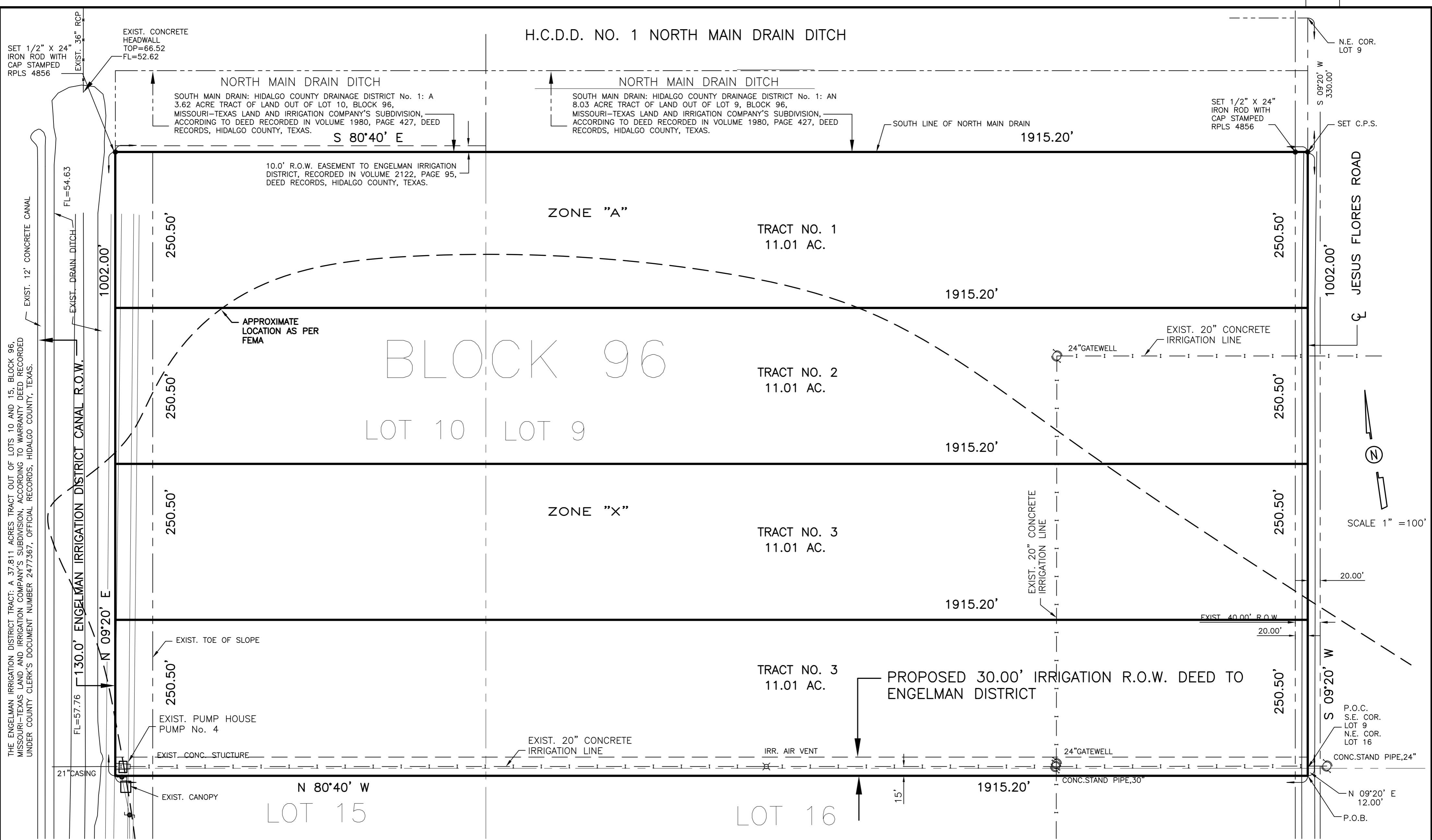
PLAT SHOWING FOUR TRACTS OUT OF A 44.05 ACRE TRACT OF LAND BEING A PART OR PORTION OF LOTS 9, 10, 15 AND 16, BLOCK 96, MISSOURI-TEXAS LAND AND IRRIGATION COMPANY'S SUBDIVISION, HIDALGO COUNTY, TEXAS, ACCORDING TO THE MAP OR PLAT THEREOF RECORDED IN VOLUME 1, PAGE 29, MAP RECORDS, HIDALGO COUNTY, TEXAS, AND ACCORDING TO WARRANTY DEED WITH VENDOR'S LIEN RECORDED UNDER COUNTY CLERK'S DOCUMENT NUMBER 1194860, OFFICIAL RECORDS, HIDALGO COUNTY, TEXAS.
